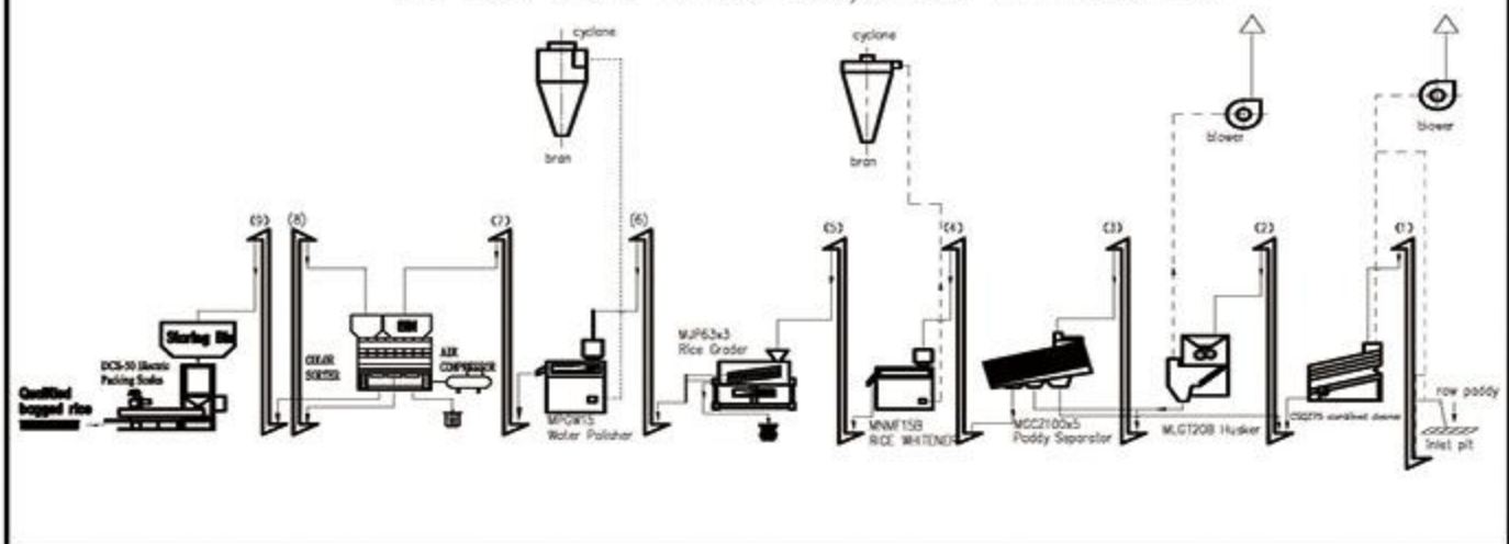
The flow chart for 20-30t/d rice mill machines
